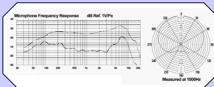
MICROPHONE FREQUENCIES
